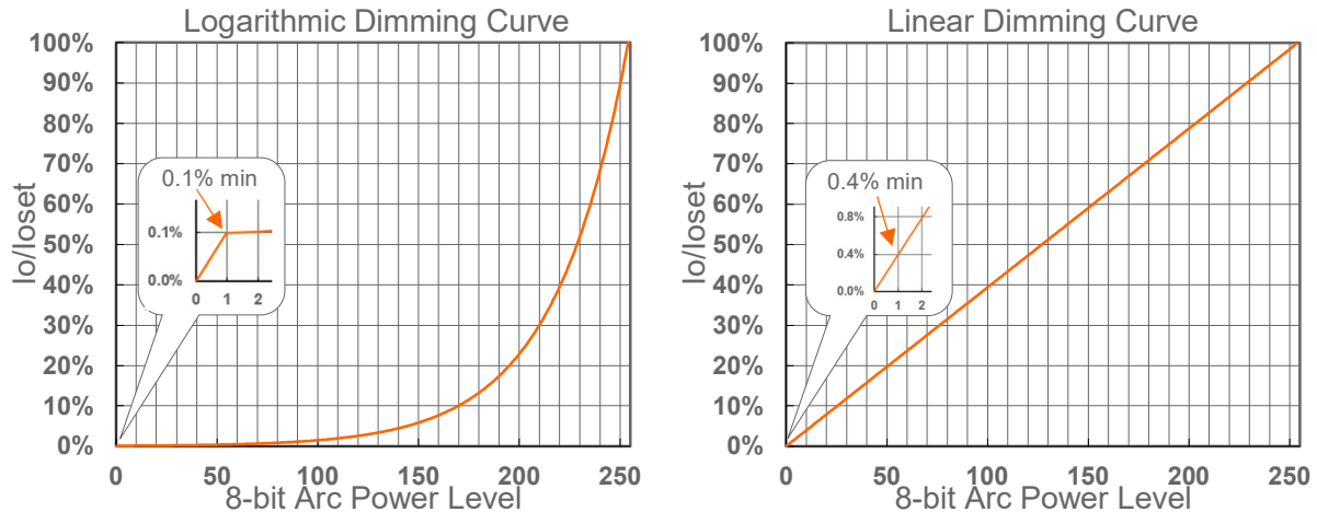
Implementation: DMX-RDM Dimming
