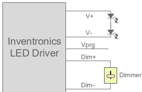
Implementation 4: Positive logic
