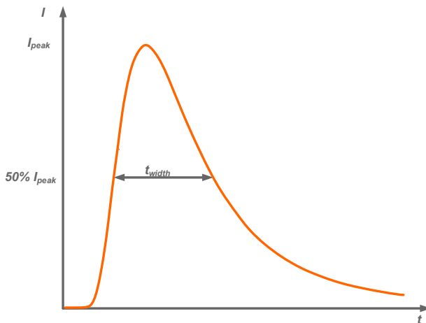
SSM-220S530HF ( I_o=4100mA )
