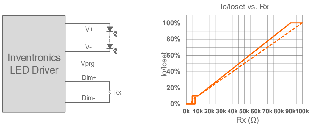
Implementation 3: Positive logic
