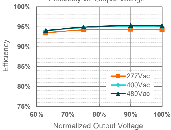
SSM-440S920HF ( I_o=8200mA ) Efficiency vs. Output Voltage
