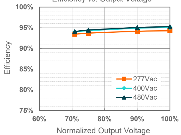
SSM-440S920HF ( I_o=9200mA ) Efficiency vs. Output Voltage
