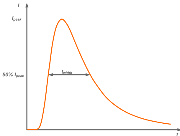
SUM-440S920HF ( I_o=8200mA )
