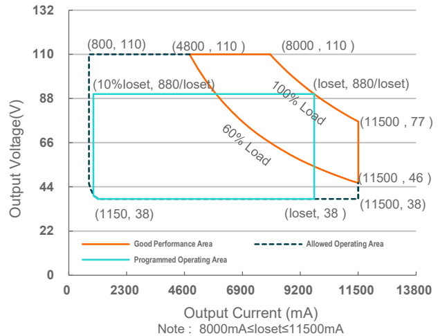
ESM-880S11AMGS
