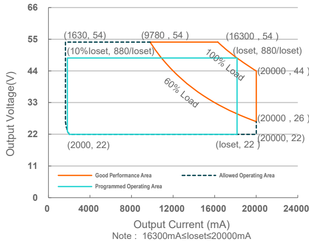
ESM-880S20AMGS
