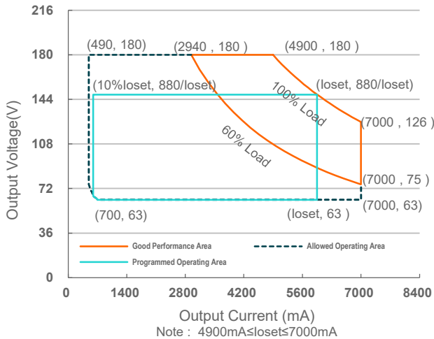
ESM-880S700MGS
