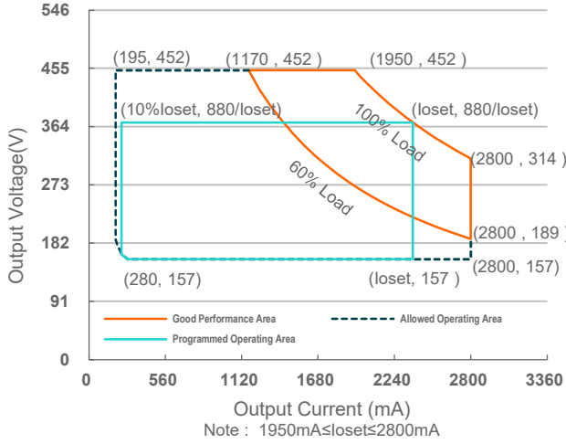
ESM-880S700MGS
