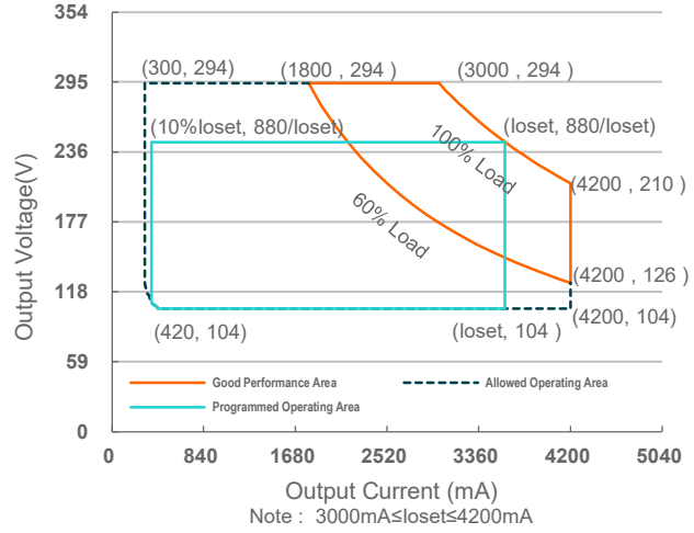
ESM-880S11AMGS
