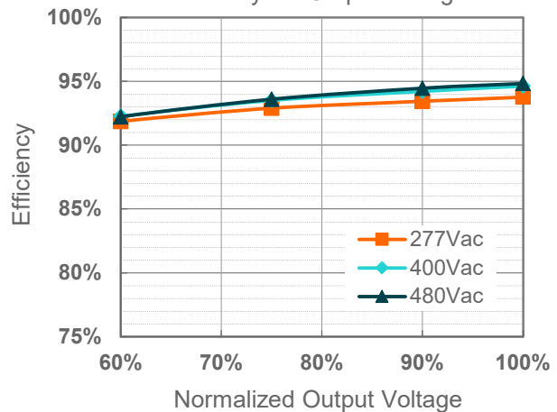
ESM-680S170MGS( I_o=1700mA ) Efficiency vs. Output Voltage
