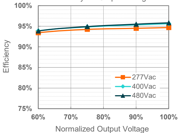
ESM-680S170MGS( I_o=1250mA ) Efficiency vs. Output Voltage
