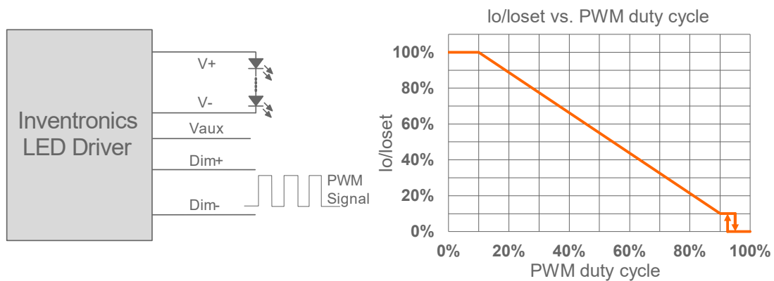
Implementation 4: Negative logic
