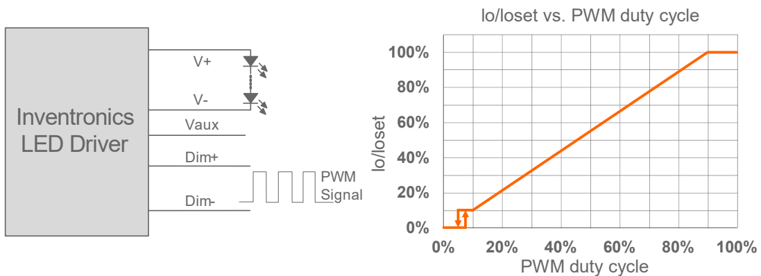
Implementation 3: Positive logic
