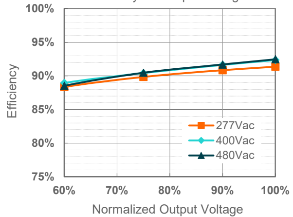
ESM-150S150Mx( I_o=1500mA )
