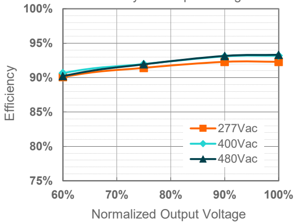
ESM-150S150Mx( I_o=1050mA )
