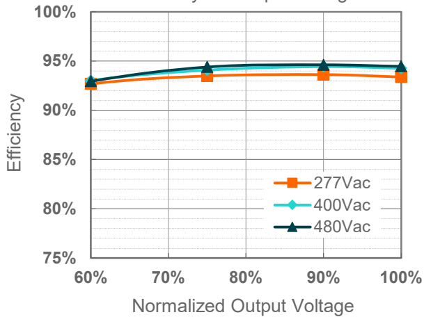
ESM-680S15AMx( I_o=12600mA ) Efficiency vs. Output Voltage
