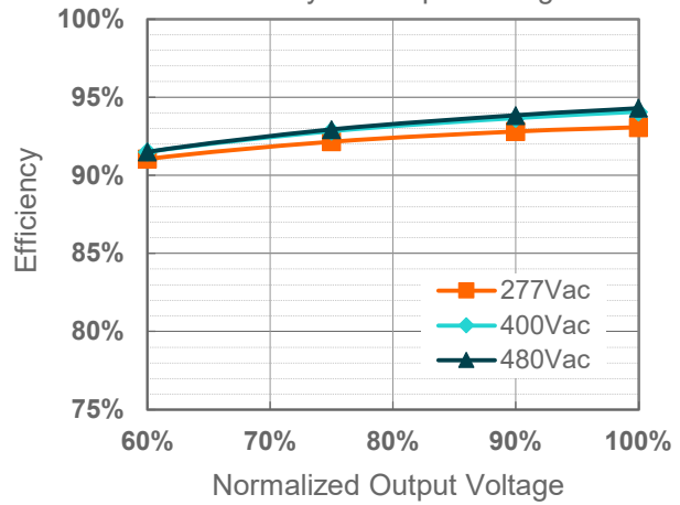
ESM-680S840Mx( I_o=8400mA ) Efficiency vs. Output Voltage
