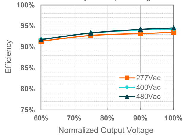
ESM-680S15AMx( I_o=15000mA ) Efficiency vs. Output Voltage
