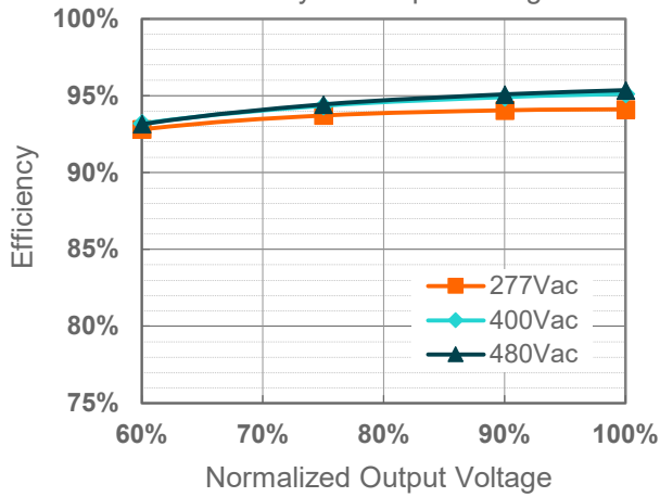
ESM-680S840Mx( I_o=6300mA ) Efficiency vs. Output Voltage
