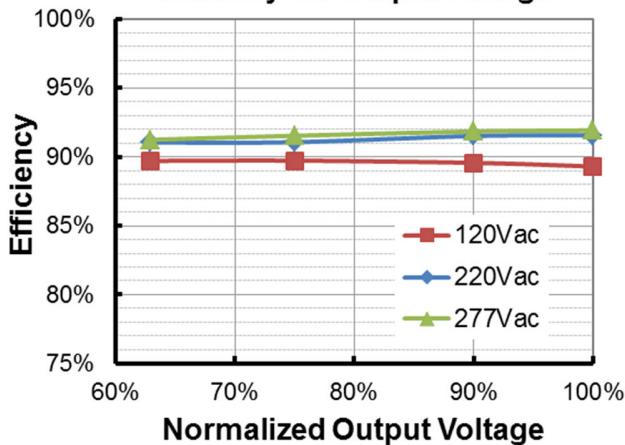
EUR-160S420Dx(Sx) (Io=3000mA) Efficiency vs. Output Voltage
