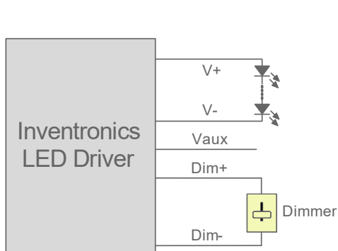
Implementation 3: Positive logic
