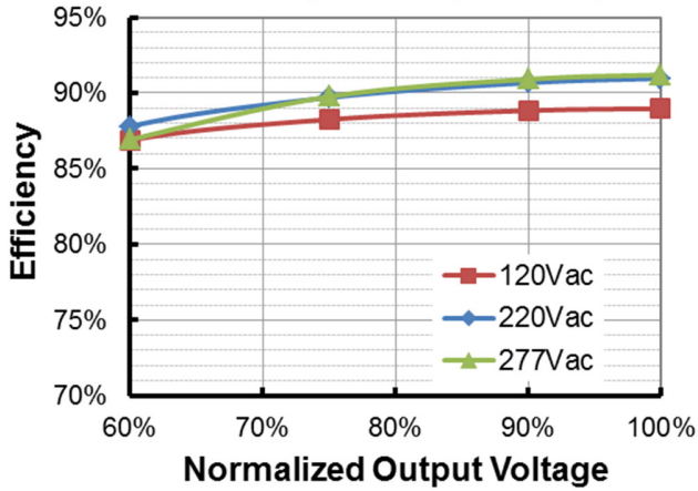
EUD-096S215DTL (I o =1750mA) Efficiency vs. Output Voltage
