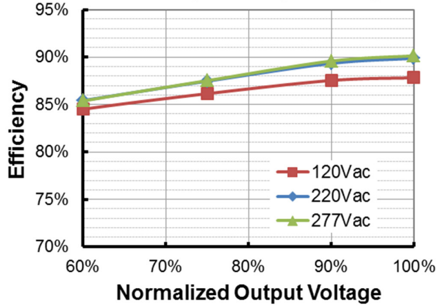
EUD-096S215DTL (I o =2150mA) Efficiency vs. Output Voltage
