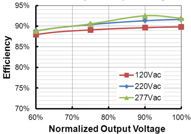
EUD-096S350DTL (I o =2450mA) Efficiency vs. Output Voltage
