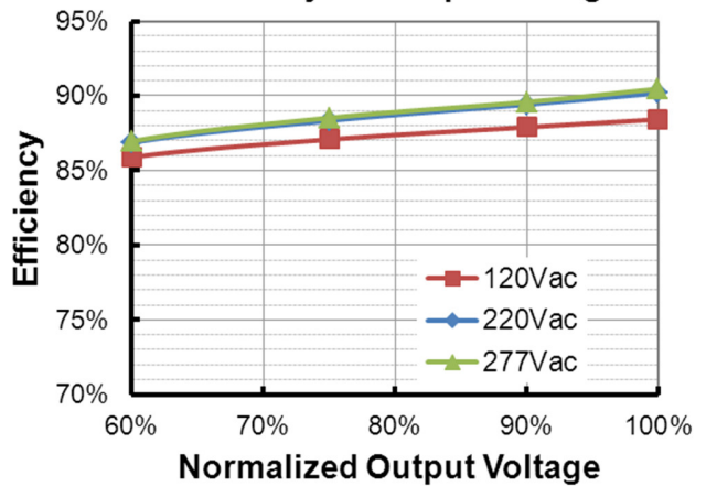
EUD-096S350DTL (I o =3500mA) Efficiency vs. Output Voltage
