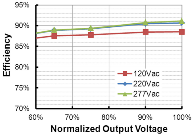
EUD-075S175DV (Io=1190mA) Efficiency vs. Output Voltage
