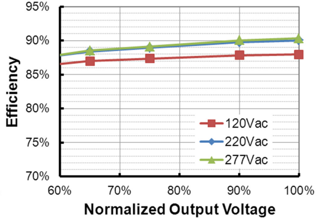
EUD-075S175DV (Io=1750mA) Efficiency vs. Output Voltage
